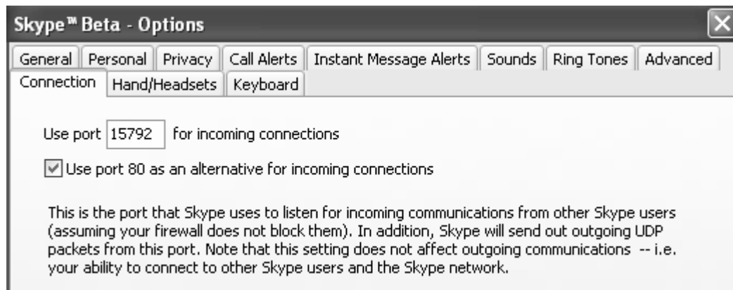
Figure 16. Skype connection tab. It shows the ports on which Skype listens for incoming connections.
